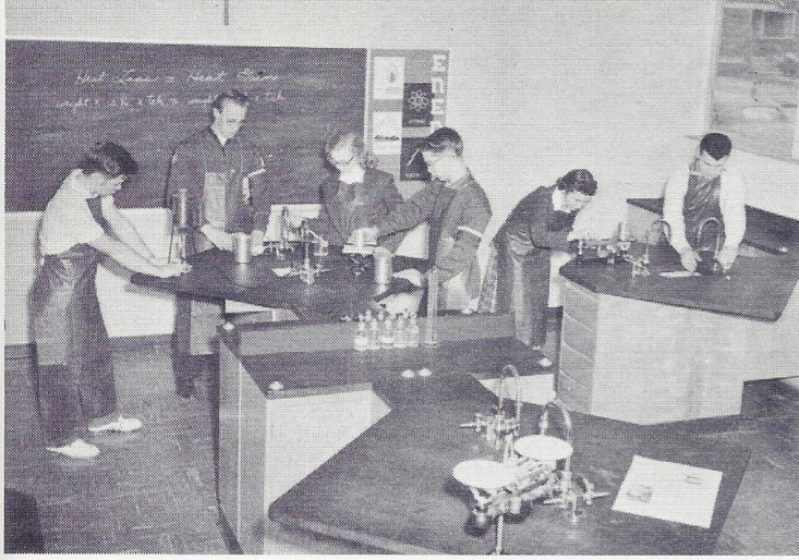
Physicists completing a heat experiment find science more absorbing than the camera. Terry Semanko, Ted Green, Jean Carlson, Albie Nephew, Jean Macy, and Kent Hultner are the studious sextet.
